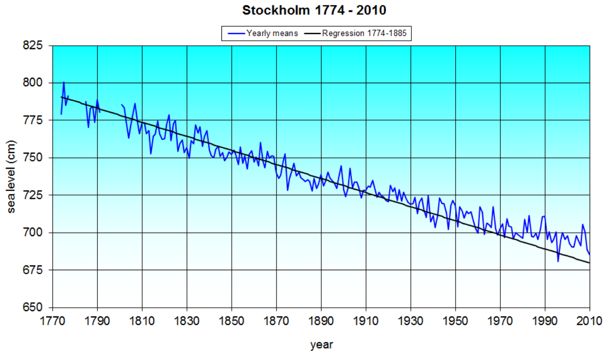
Figure 3. Annual mean sea levels in Stockholm since 1774, with the regression line (corresponding to land uplift) for 1774-1885 and its extension into modern times. The increased sea level rise since the late 19 th century appears as a deviation from the regression line.
