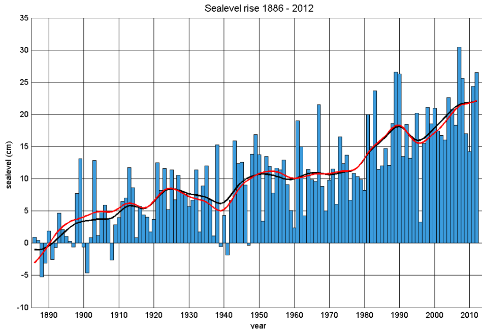
Figure 6. Sea levels corrected for the absolute land uplift (isostatic adjustment). Blue bars show the annual sea level averaged for 14 Swedish sea level records, compared to the 1886 level. The black and red line shows the gauss-filtered average and Stockholm sea level, respectively.
